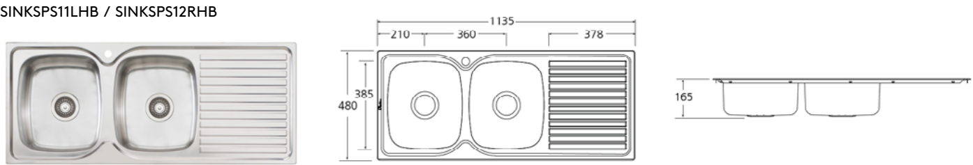
SINKSPS11LHB / SINKSPS12RHB
