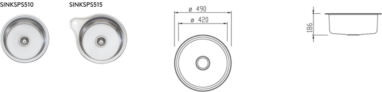
SINKSPS510
