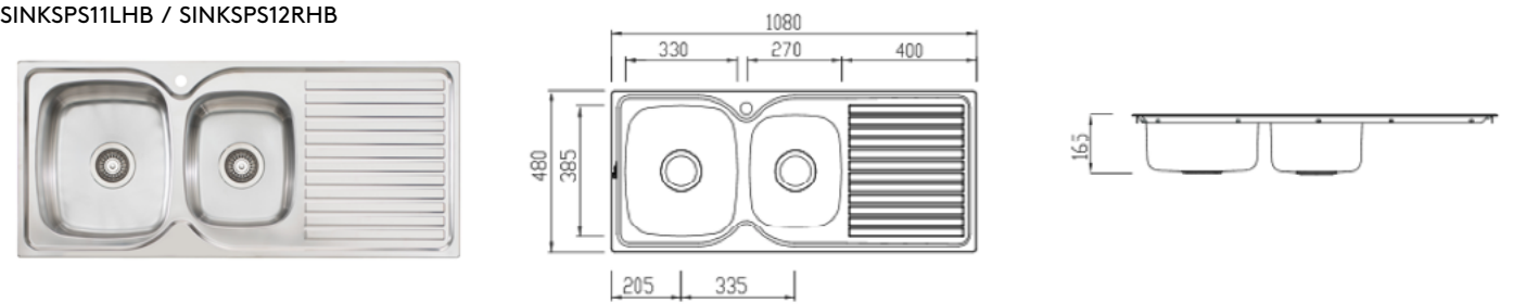
SINKSPS11LHB / SINKSPS12RHB
