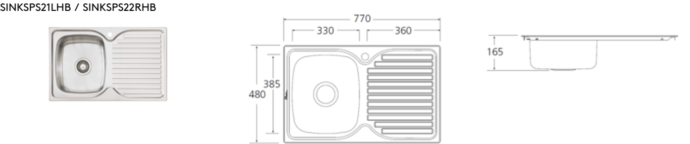
SINKSPS21LHB / SINKSPS22RHB
